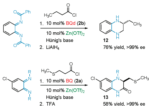
SCHEME 10. Synthesis of Drug Targets, R = CO 2 -i-Pr
