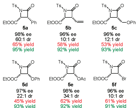
FIGURE 1. Sample of \beta -lactams synthesized, employing cocatalysts BQ and \text{In}(\text{OTf})_3 (yields in red without metal).
