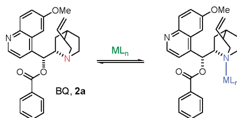
SCHEME 3. Cocatalyst Quenching
